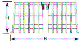
LEAF GRATE and/or GRAVEL GRATE
